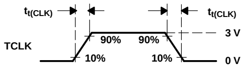
Figure 6. Serializer Input Clock Transition Time
