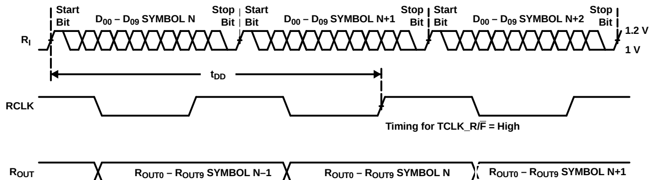
Figure 12. Deserializer Delay
